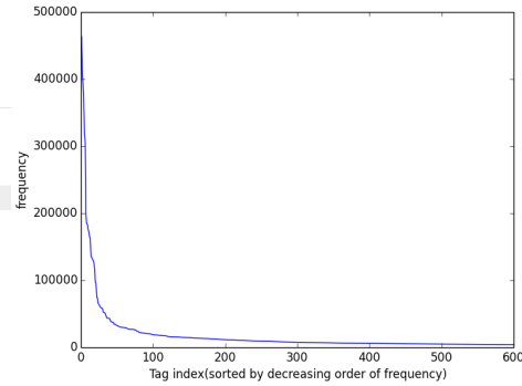
Fig. 2: Tag Frequency distribution(top 600 tags)
